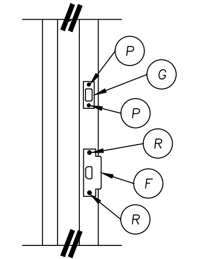
STRIKE PLATE DETAIL ANSI STRIKE & DEADBOLT
