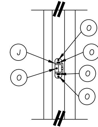
RIM STRIKE DETAIL
