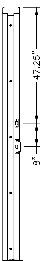
STRIKE PLATE LOCATIONS 2" HEAD
