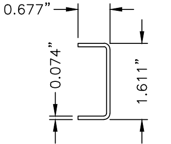
1 DOOR STILE EDGE REINFORCEMENT
