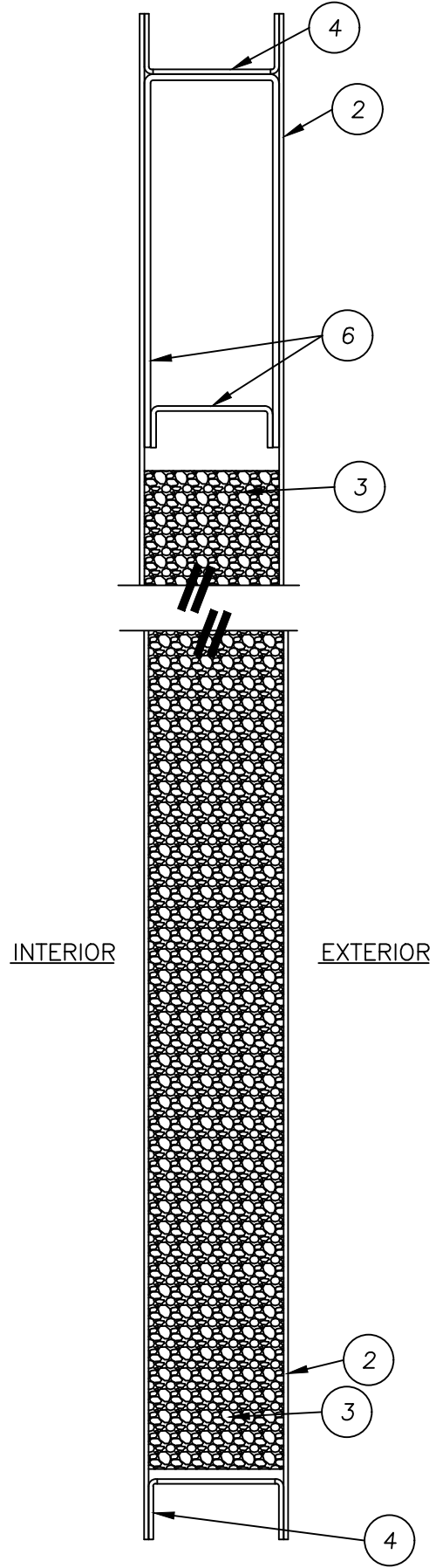
1/2 VERTICAL CROSS SECTION
