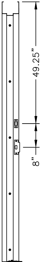
STRIKE PLATE LOCATIONS 4" HEAD
